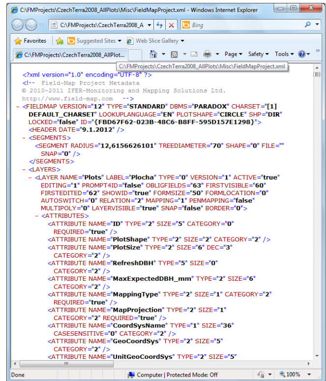
Example of FieldMapProject.xml
